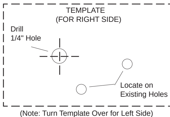
Template for Eye Bolt Assembly
